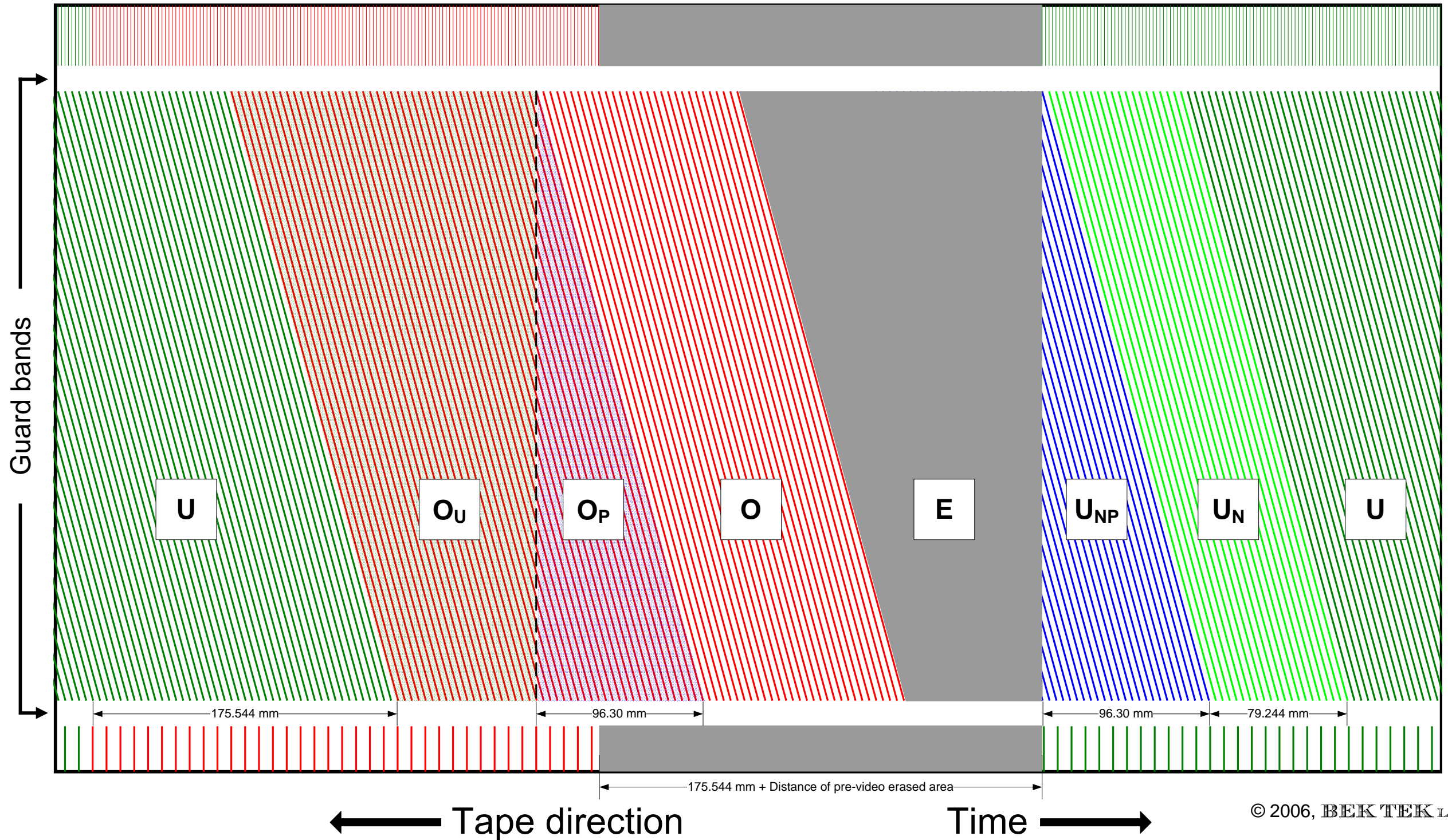
Figure 5b: Color-coded representation of a longer overrecording on a VCR at SP speed, with the vertical dimension enlarged 35 times. This VCR does not have a flying erase head.
