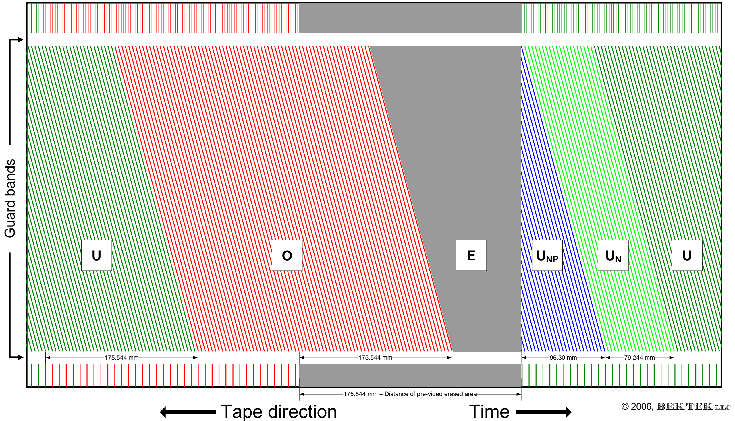
Figure 5a: Color-coded representation of a longer overrecording on a VCR at SP speed, with the vertical dimension enlarged 35 times. This VCR has a flying erase head.
