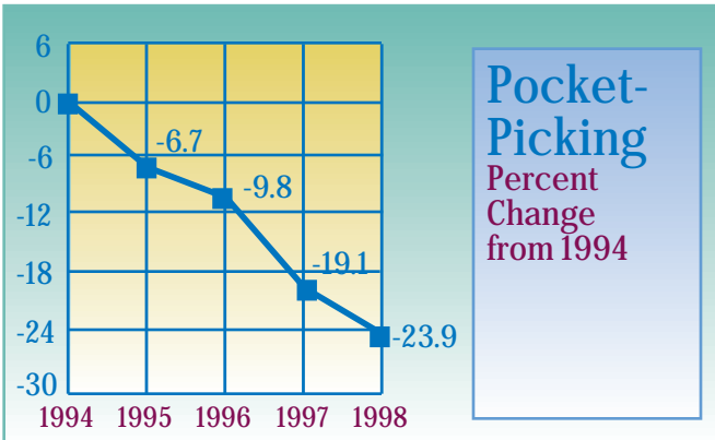
Figure 2.15 Larceny-Theft Analysis
